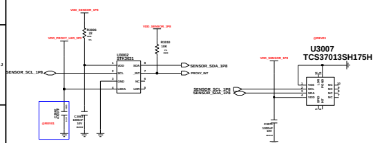
Proxi Sensor
